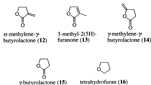
Chart 3. Chemical structures of \gamma -butyrolactones and a related compound.
